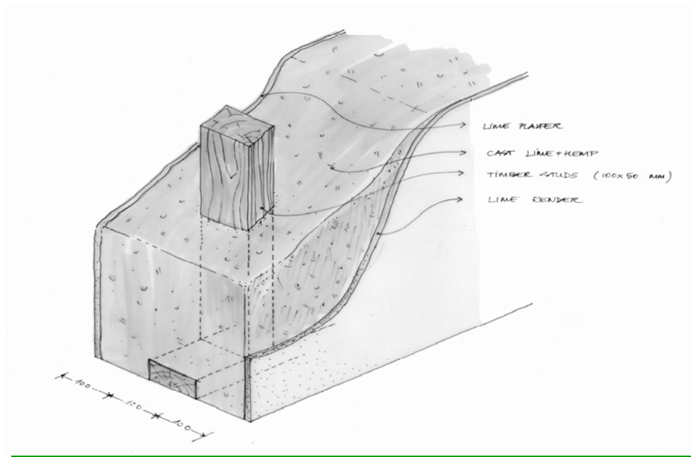
Figure 2: Hempcrete Wall. Source: Ian Pritchett (CAT 2006).
