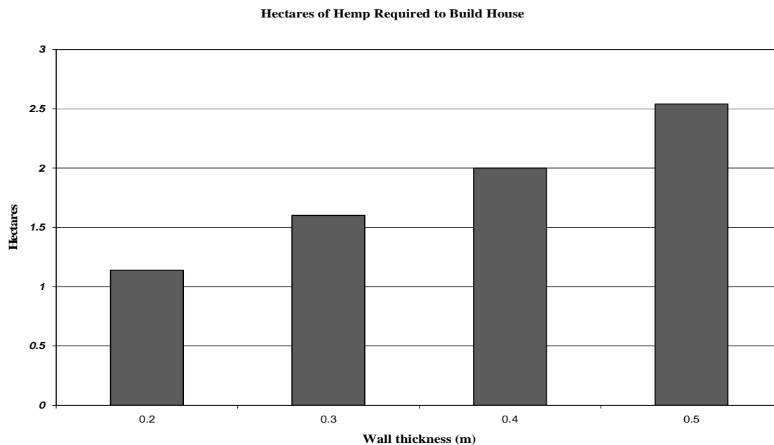
Figure 3: Area required against thickness of wall. Source: this author.
