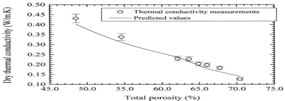
Figure 1: The effect of porosity. Source: Bouguerra (1998).
